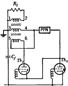
FIG. 11-40.—Circuit diagram for a double-switch single-network pulser.
